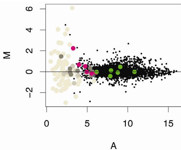
Figure 2 Cadmium effects on gene expression: Buffers, blanks, and controls. Gene expression data from control and cadmium (20 µg Cd/L for 48-h) treated Daphnia pulex [GEO:GSE9746]. Data were LOESS normalized; duplicate probes were averaged within LIMMA using gene-wise linear models fit to expression data, and gene expression log ratios ( M = \log_2 \text{treated/control} ) were plotted against log mean intensity values ( A = 1/2 \log_2 (\text{treated} * \text{control}) ). Print control elements (buffers, blanks, betaine; grey shades); negative controls (non-daphniid cDNA; pink); and positive controls ( D. pulex cytochrome b and c, actin, and ferritin; green) are highlighted.
