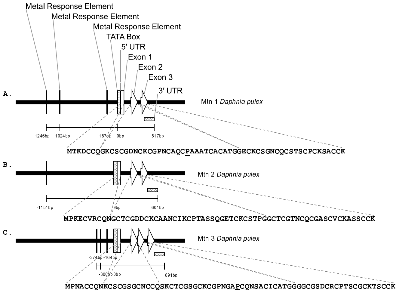
Figure 6 Metallothionein gene models. Daphnia pulex metallothionein gene models. A) Dpu Mtn1 [GenBank:EU307302], B) Dpu Mtn2 [GenBank:EU307303], and C) Dpu Mtn3 [GenBank:EU307304].
